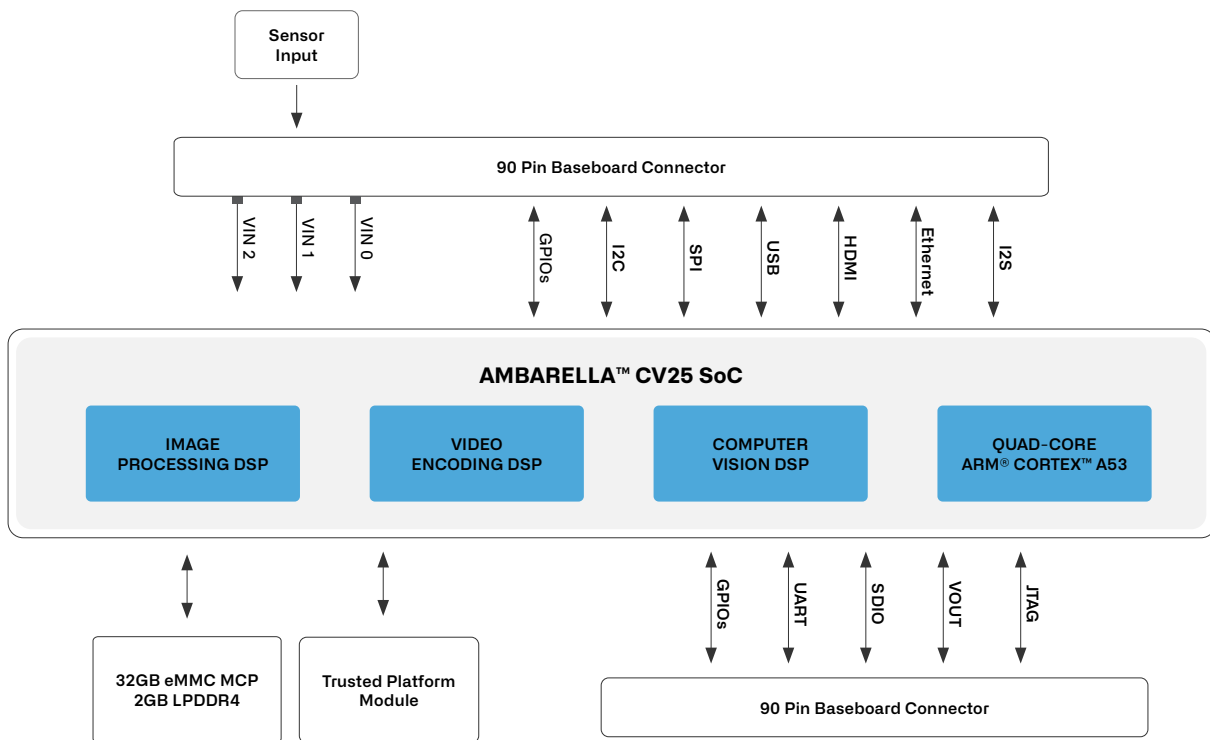
The Oclea™ CV25 μSoM Block Diagram
